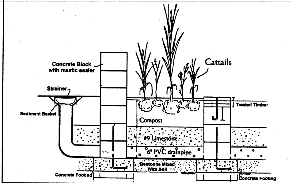
Cross Section of Passive Treatment System (from University of Kentucky, Department of Agronomy)
