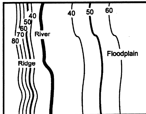
3. Contour Lines
