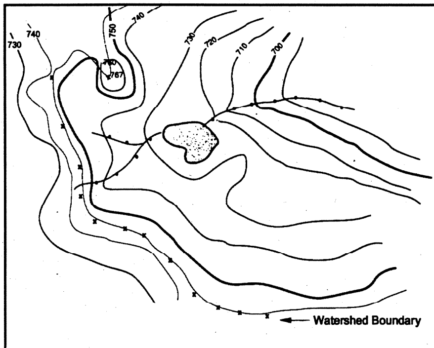
Topographic Map
