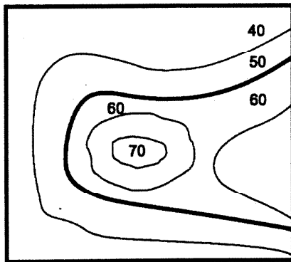
3. Contour Lines
